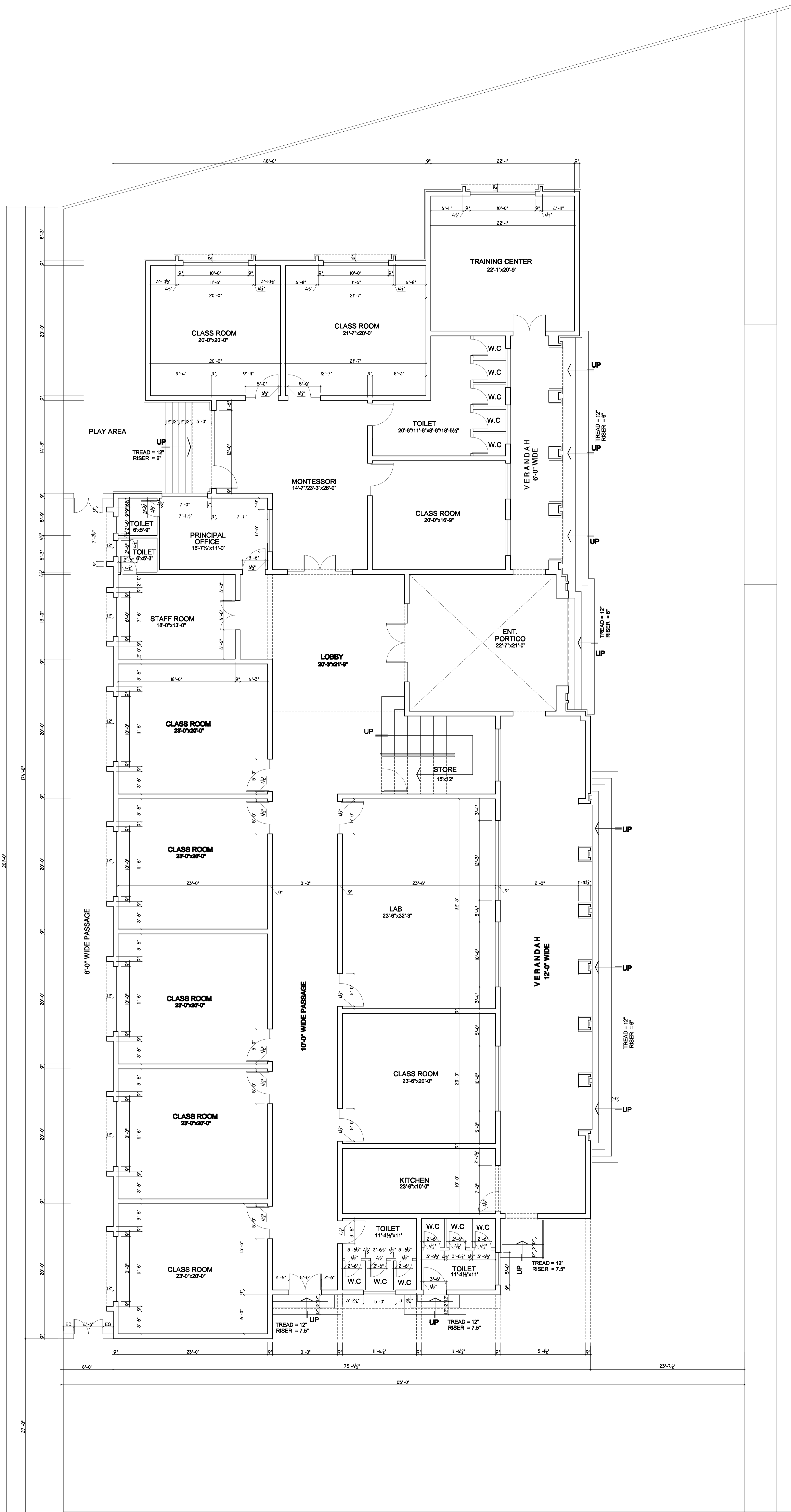
GROUND FLOOR PLAN AREA 10,112 SFT SCALE 1/8" = 1'-0"
